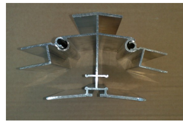
Ridge Connection for Polycarb
